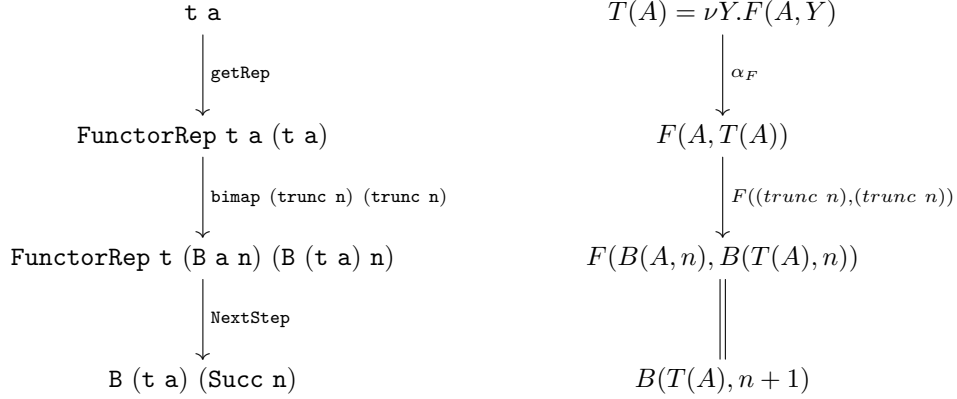
■ Figure 2 Generic definition of truncations in Haskell
