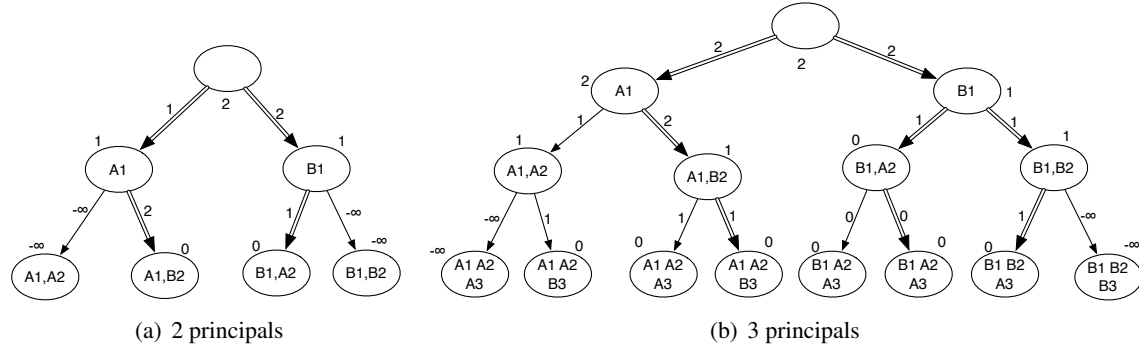
Figure 5: Join transitions of KSL
