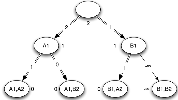
Figure 4: Weighted states in NS
