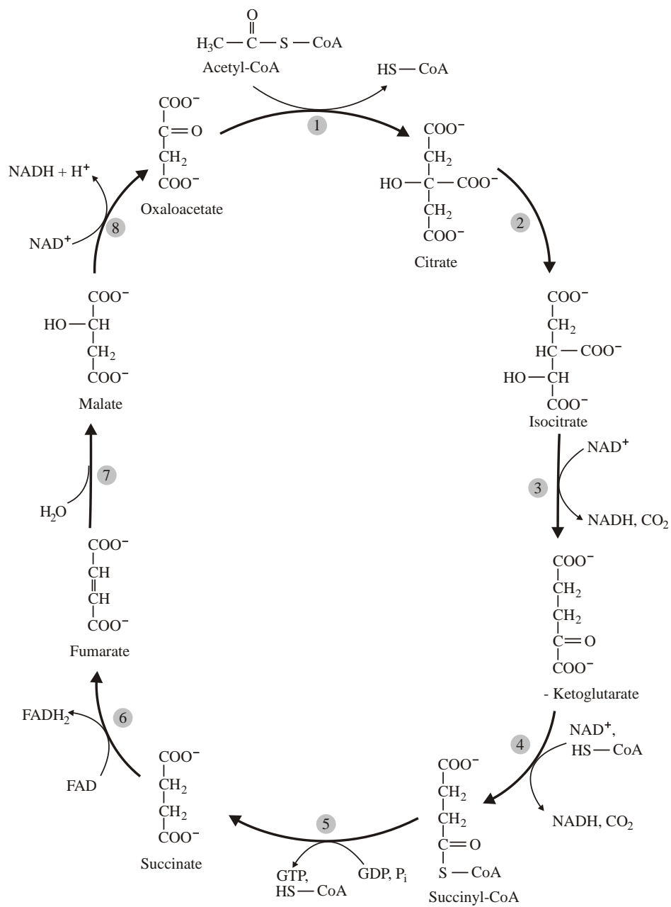
Fig. 1. Citric Acid Cycle
