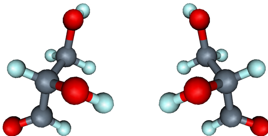
Fig. 5. 3-dimensional view of L-glyceraldehyde and D-glyceraldehyde (from left to right), created with MolSurf www2.chemie.uni-erlangen.de/services/mol surf/ .
