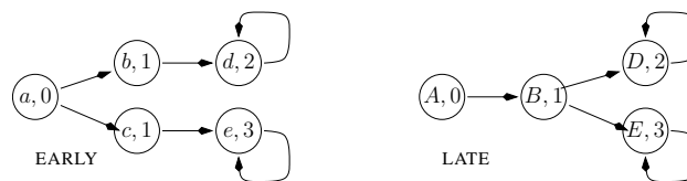
Fig. 1. Systems EARLY and LATE
