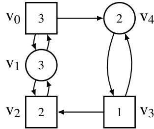
Figure 1: A parity game with winning regions W_0 = \{v_1, v_2\} and W_1 = \{v_0, v_3, v_4\} ; winning strategies for players 0 and 1 map v_1 to v_2 , respectively v_0 and v_3 to v_4
