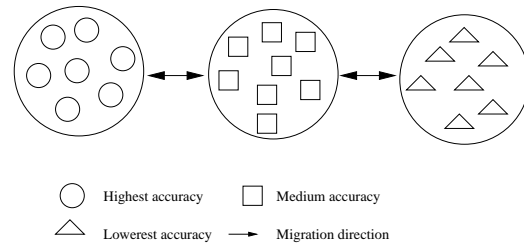
Fig. 2 Hierarchical GA for incorporating approximate fitness models.
