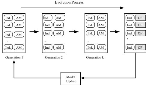
Fig. 5 Generation-based evolution control. AM: approximate model; OF: original function.
