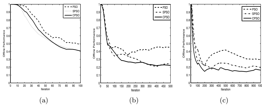
Fig. 4. Dynamic performance of PSOs on dynamic problems with s = 1.0 : (a) \tau = 10 , (b) \tau = 50 , and (c) \tau = 100
