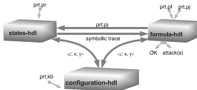
Fig. 1. ASPASyA architecture
