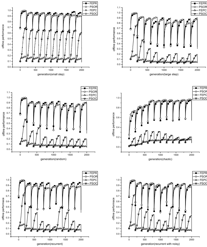
Fig. 2. The offline performance of PSO and FEP in the composition and rotation DBG environments
