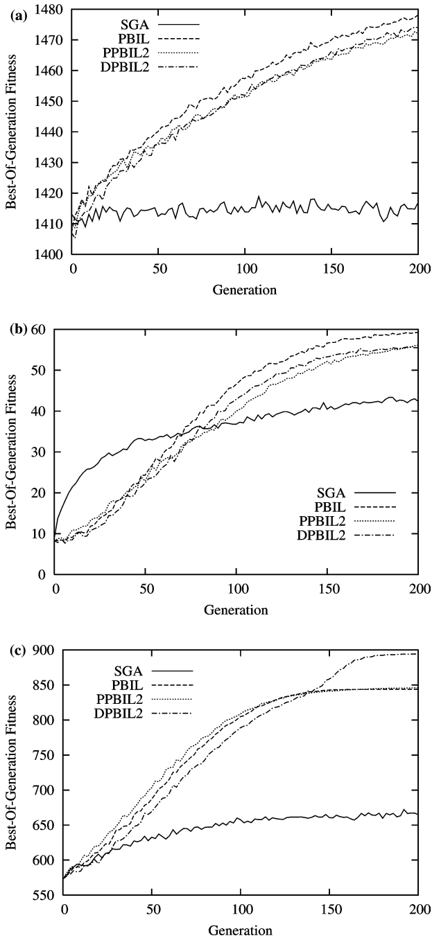
Fig. 5 Experimental results with respect to best-of-generation fitness against generations of algorithms on stationary problems: a Knapsack, b Royal road, and c Deceptive. The data were averaged over 50 runs
