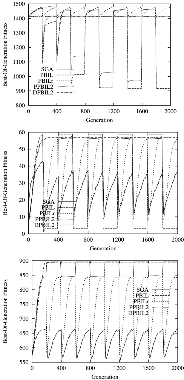
Fig. 10 Dynamic behavior of algorithms on dynamic problems: (Top) Knapsack, (Middle) royal road, and (Bottom) Deceptive. The environmental dynamics parameter \tau is set to 200 and \rho is set to 1.0
