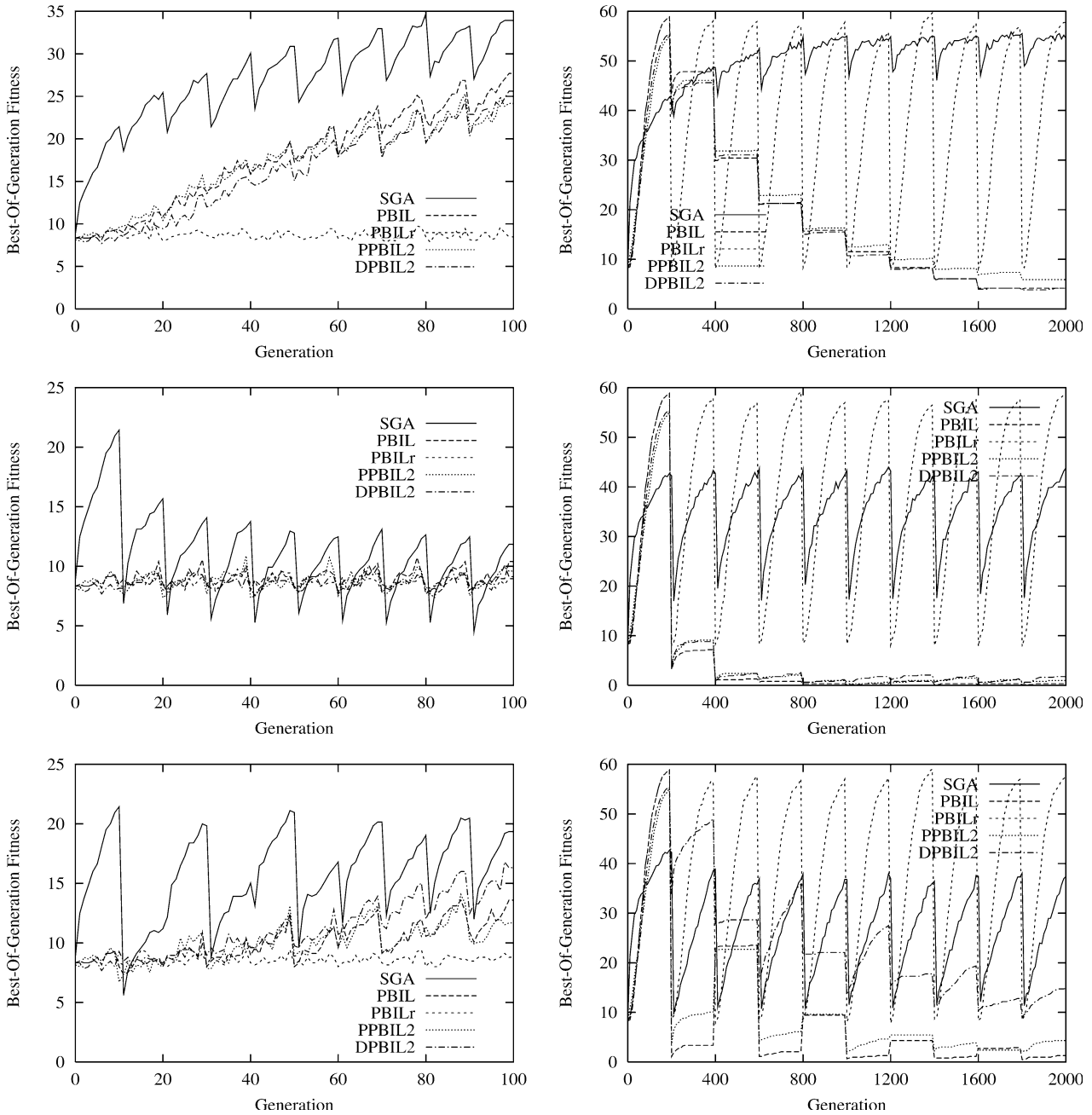
Fig. 8 Dynamic behavior of algorithms on dynamic royal road functions. The environmental dynamics parameter \tau is set to 10 (Left Column) and 200 (Right Column) respectively and \rho is set to 0.05, 0.4, and 0.95 from top to bottom row respectively
