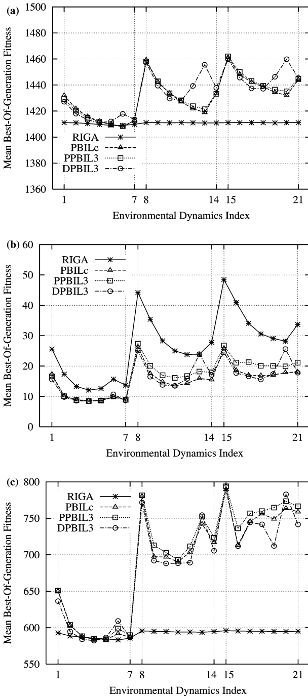
Fig. 14 Experimental results of RIGA, PBILc, PPBIL3, and DPBIL3 with respect to mean best-of-generation fitness against different environmental dynamics parameter settings on dynamic problems: a Knapsack, b royal road, and c Deceptive
