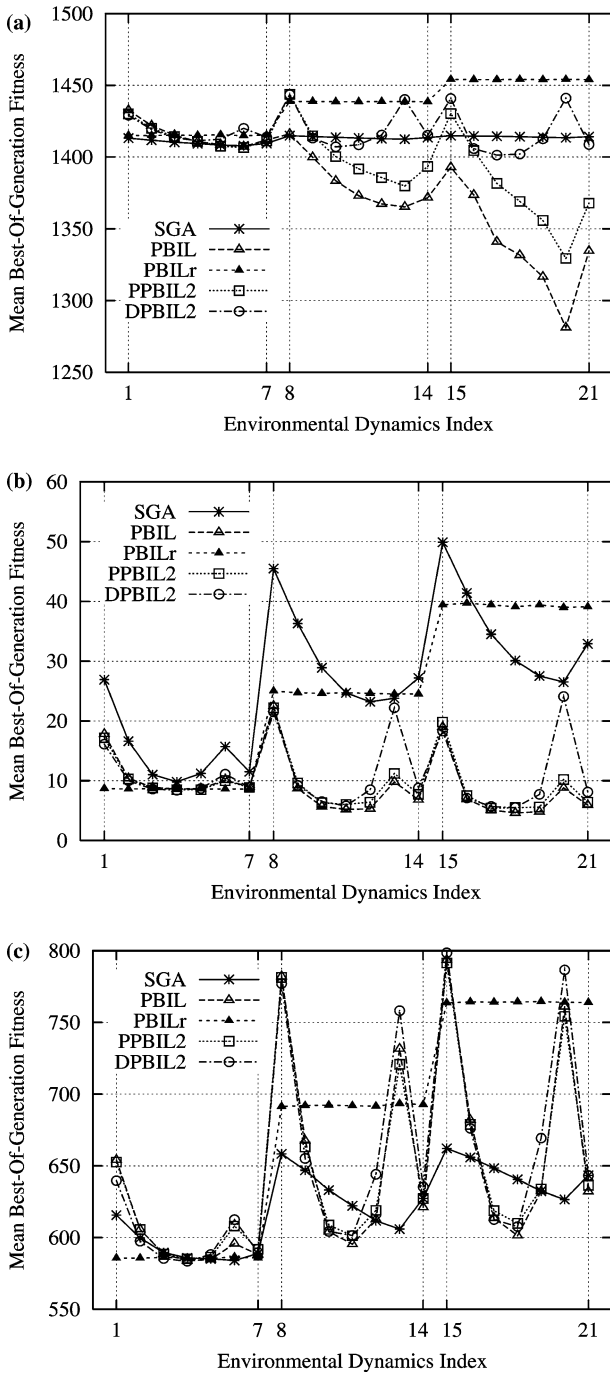
Fig. 6 Experimental results of SGA, PBIL, PBILr, PPBIL2, and DPBIL2 with respect to mean best-of-generation settings against different environmental dynamics parameter settings on dynamic problems: a Knapsack, b Royal road, and c Deceptive
