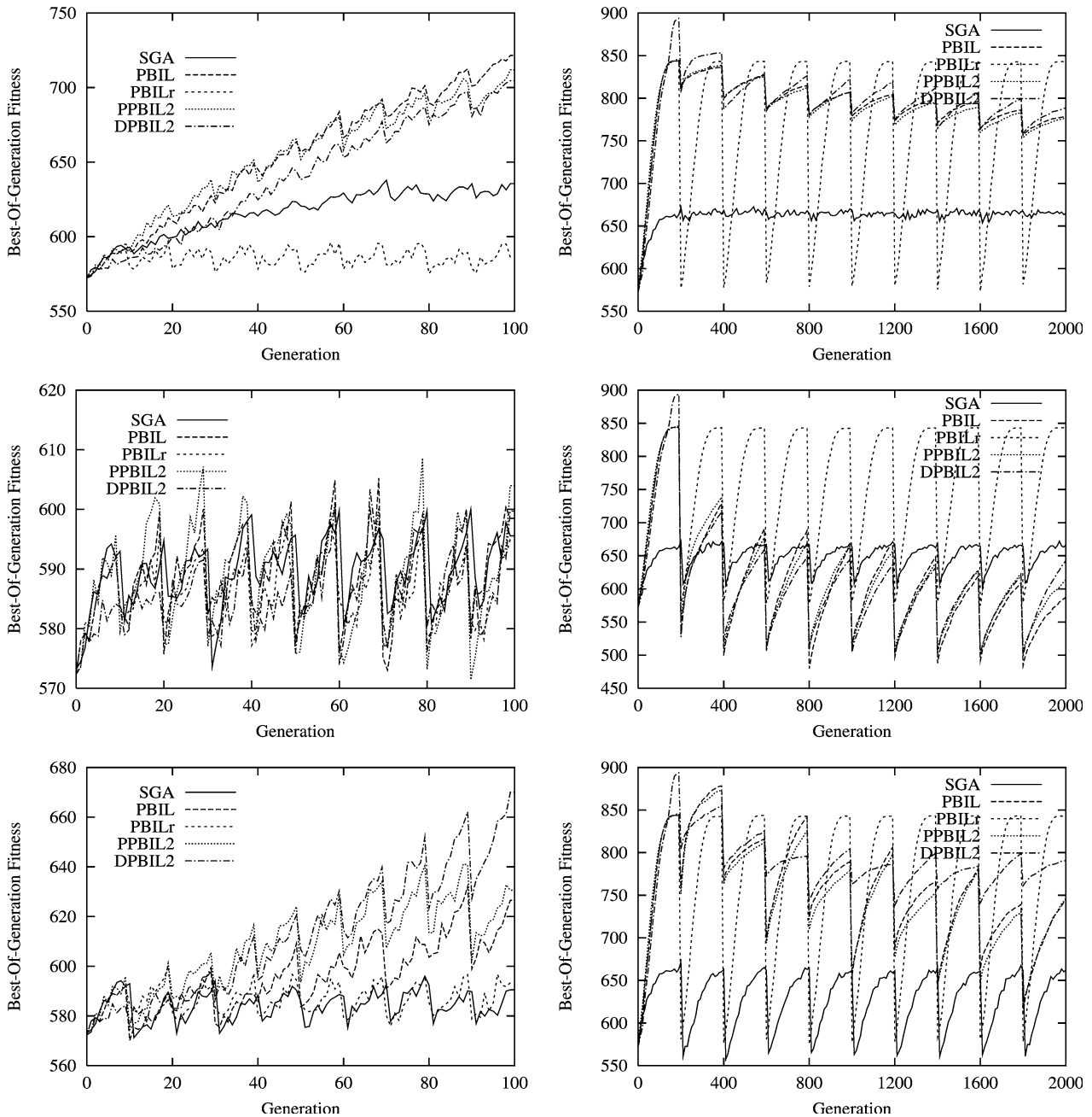
Fig. 9 Dynamic behavior of algorithms on dynamic deceptive functions. The environmental dynamics parameter \tau is set to 10 (Left Column) and 200 (Right Column) respectively and \rho is set to 0.05, 0.4, and 0.95 from top to bottom row respectively
