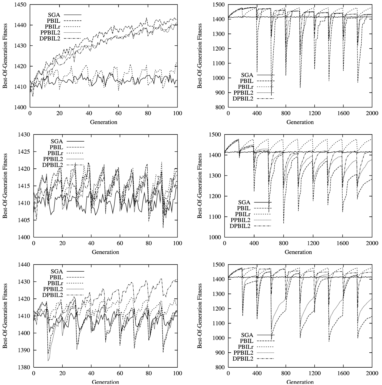
Fig. 7 Dynamic behavior of algorithms on dynamic knapsack problems. The environmental dynamics parameter \tau is set to 10 (Left Column) and 200 (Right Column) respectively and \rho is set to 0.05, 0.4, and 0.95 from top to bottom row respectively
